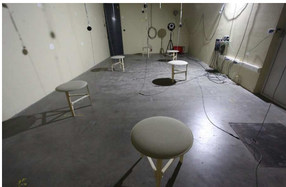
Photos top to bottom from measurement 4: SOLI – SHHH 60 - height 50 cm
