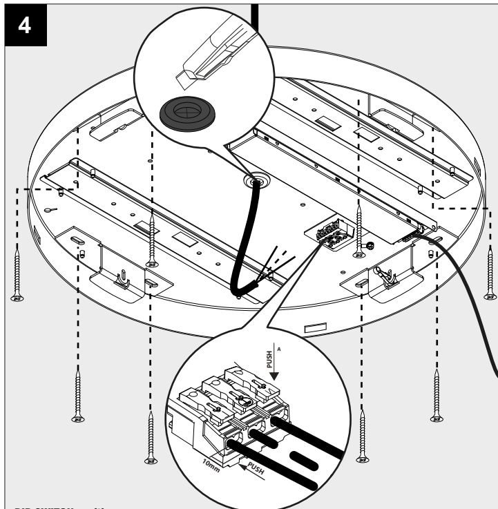
DIP SWITCH position
