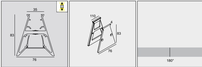
FTL35 X HE D/U - PROFILE
